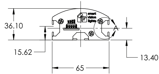
LHF300-M12 & ODLHF300-M12 option pictured at left comes with M12 pre-assembled.
