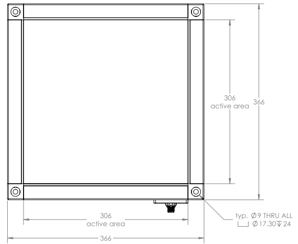
CAD drawings are 306 x 306 mm versions of LLPX.
