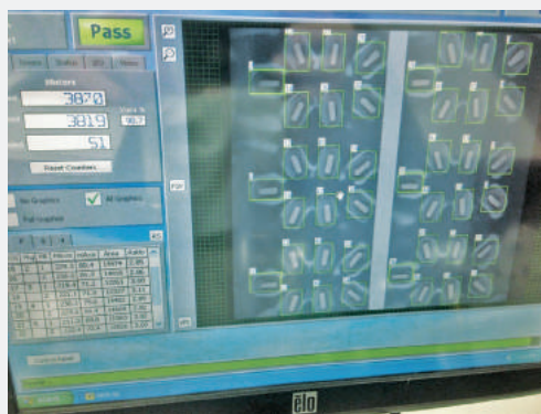
Illumination: TL305 Diffuse On & Off Axis Light
