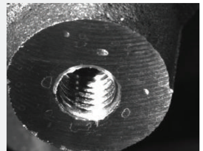
Threaded hole with white test fluid inside, potentially yielding false-negative result.
